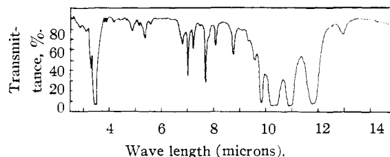
Fig. 1.—Infrared spectrum of 2-oxaspiro[3,2]hexane (liquid).
